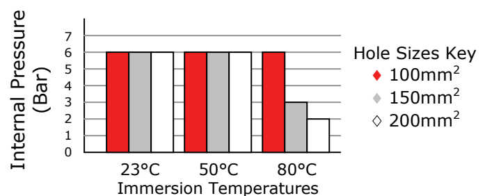
Burst pressures for various hole sizes
